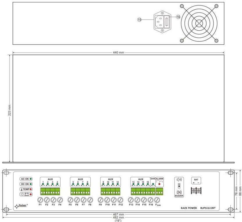
Fig.3. The view of the PSU.
